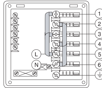
Figure 13 220-240V 1N
