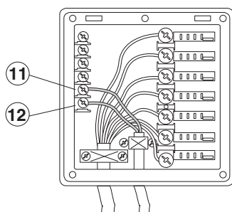
Figure 12 Energy control
