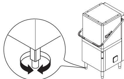
Figure 8 Feet adjustment
