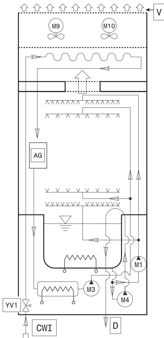
Plumbing circuit diagram - manual hood type with drain pump and energy saving device (ESD)
