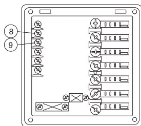
Figure 18 Rinse aid dispenser terminal block
