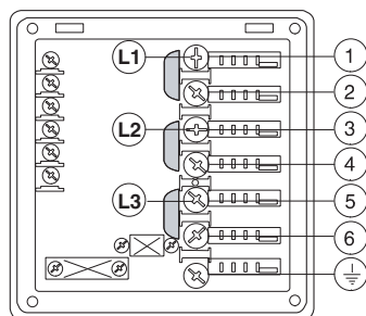
Figure 11 200V 3
