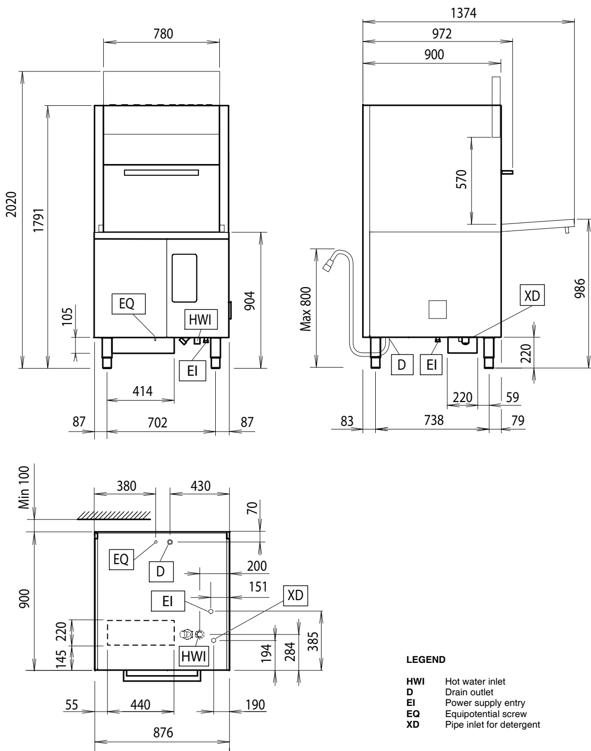
Installation diagram for EPPWES (electric versions)
