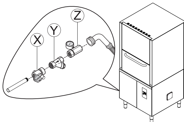
Figure 10 Feed pipe connection
