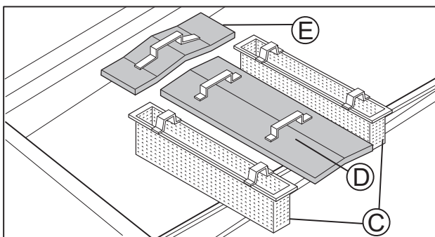
Figure 15 Tank filters
