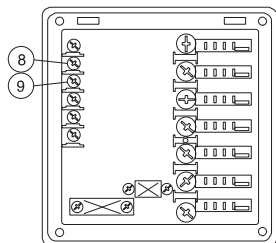
Figure 19 Rinse aid dispenser terminal block
