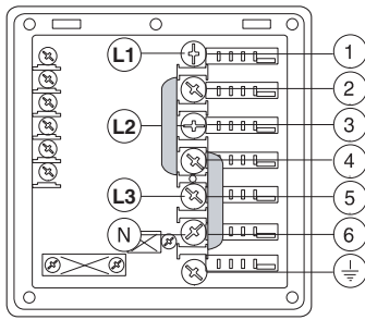
Figure 11 380-415 V 3N
