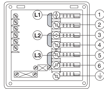
Figure 13 220-230V 3
