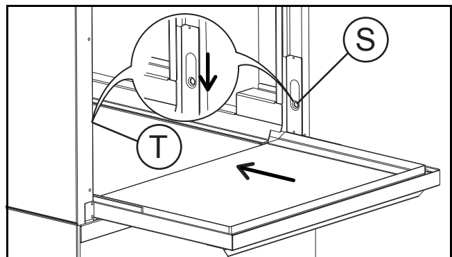
Figure 25 Refit the door
