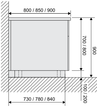
3. Against the wall on steel plinth or adjustable feet
