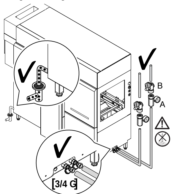
Fig. 3 Plumbing connection for left machine
