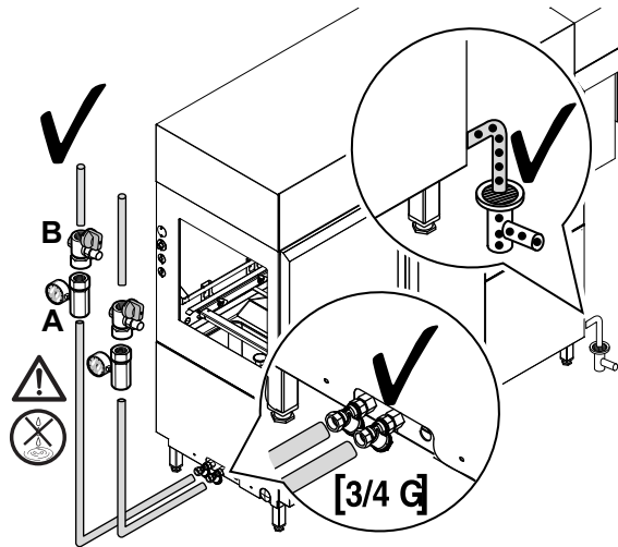
Fig. 3 Plumbing connection for left machine
