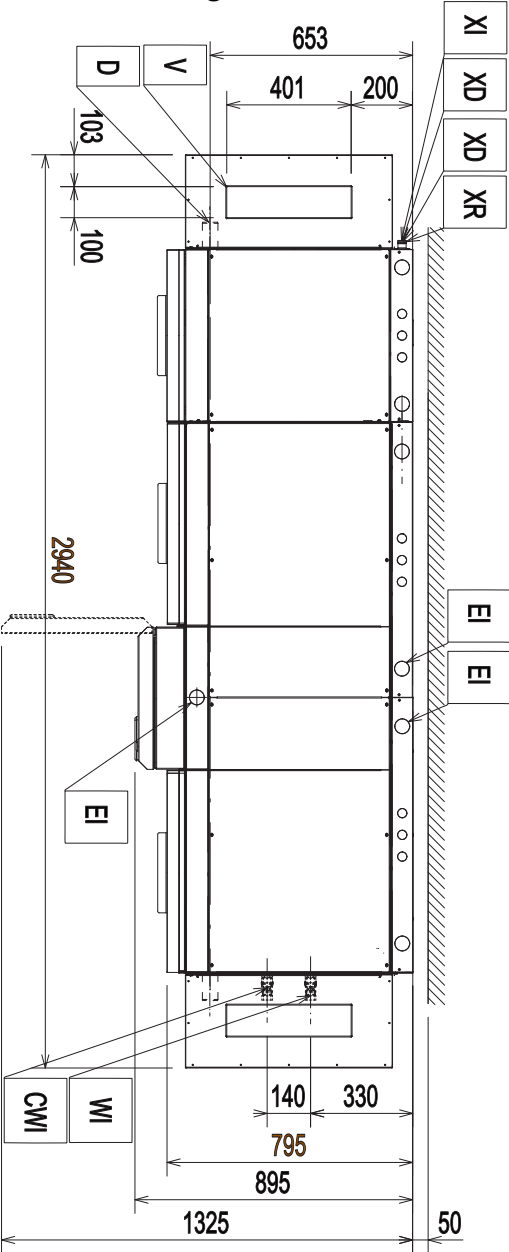
Installation diagram
