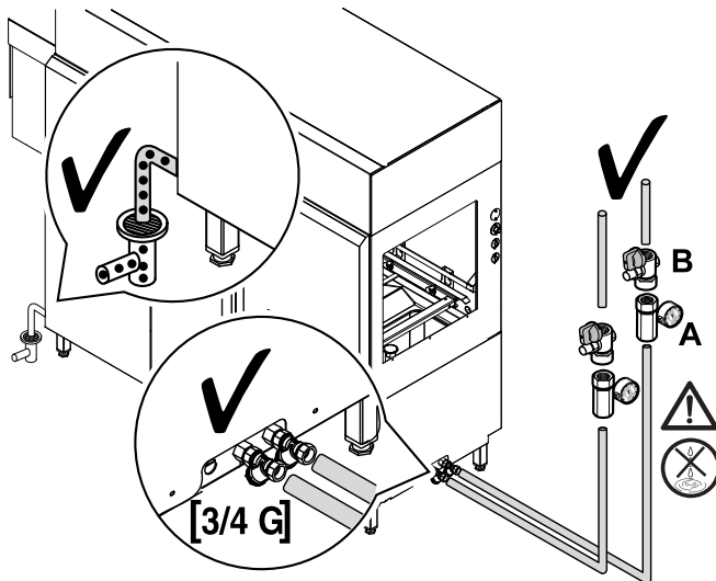
Fig. 4 Plumbing connection for right machine
