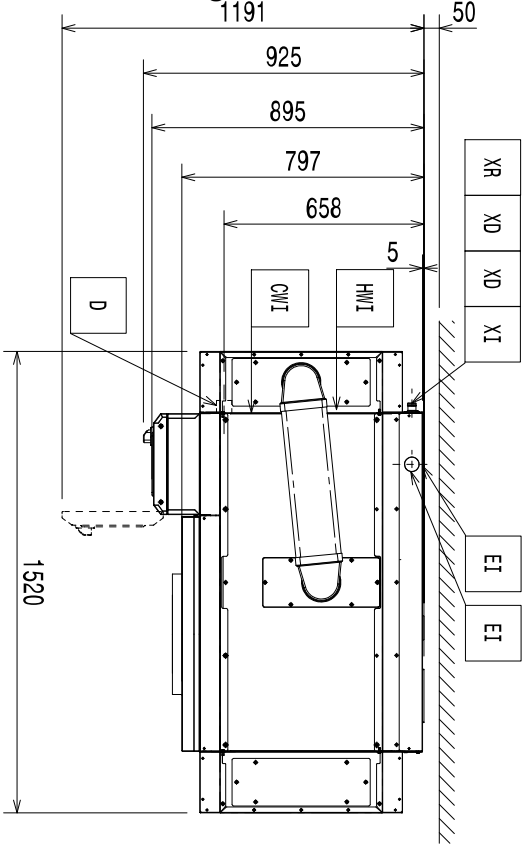
Installation diagram
