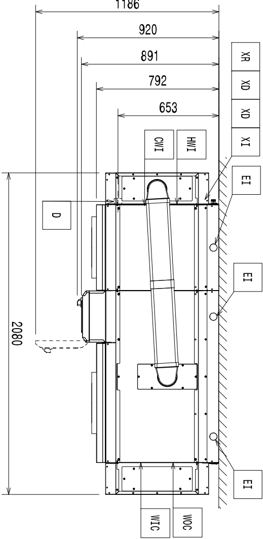
Installation diagram
