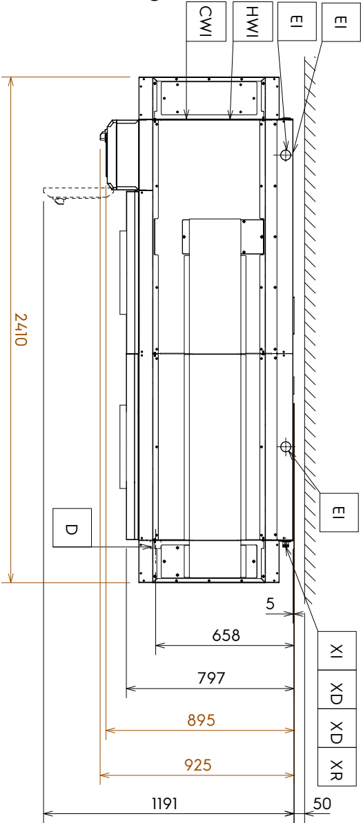
Installationsdiagram
