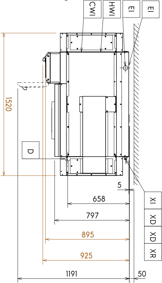
Installation diagram
