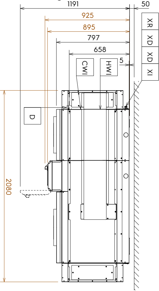
Installation diagram
