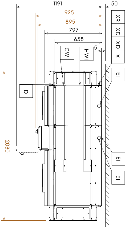
Installation diagram
