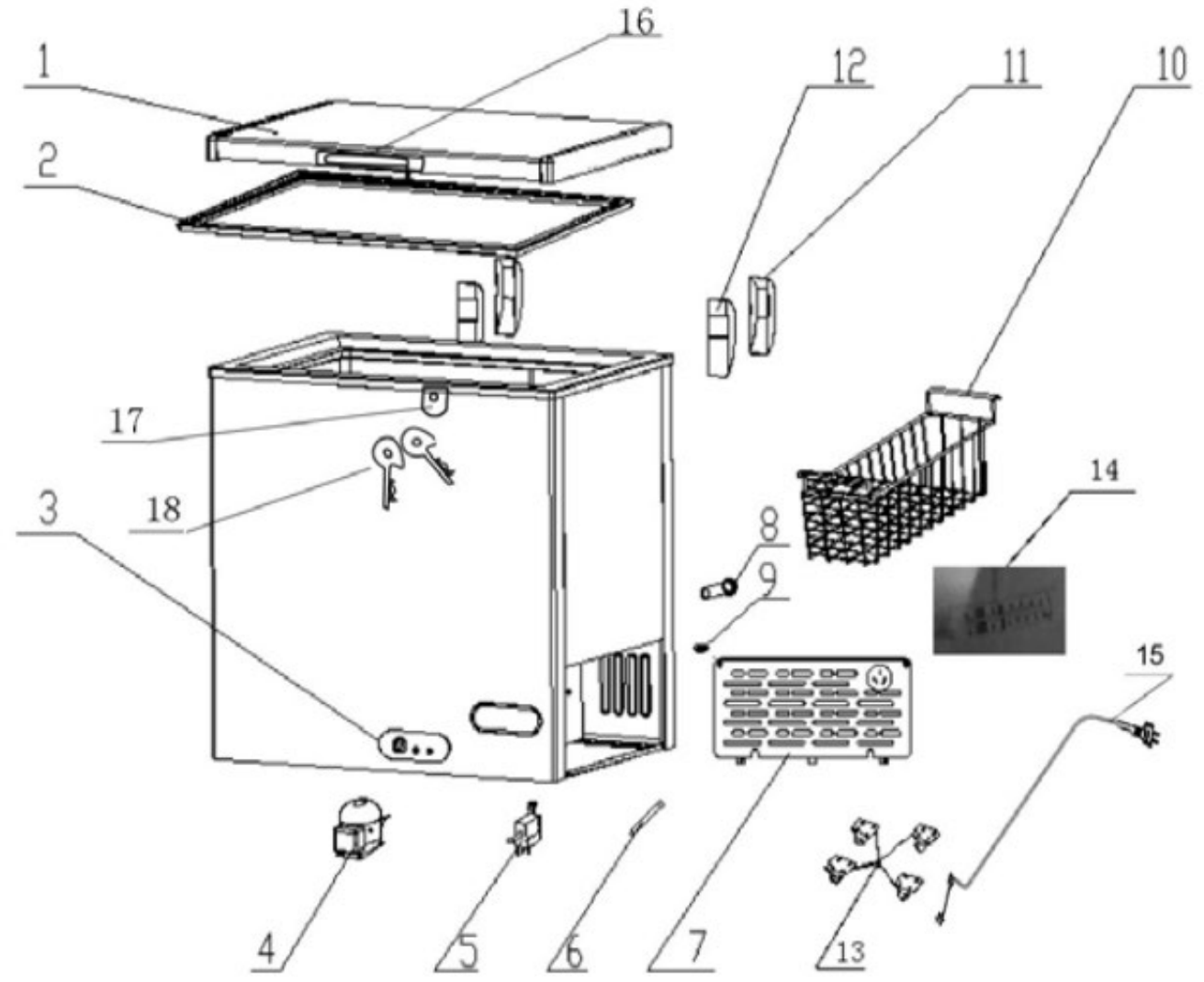
Explosion View Of KCCF073WS
