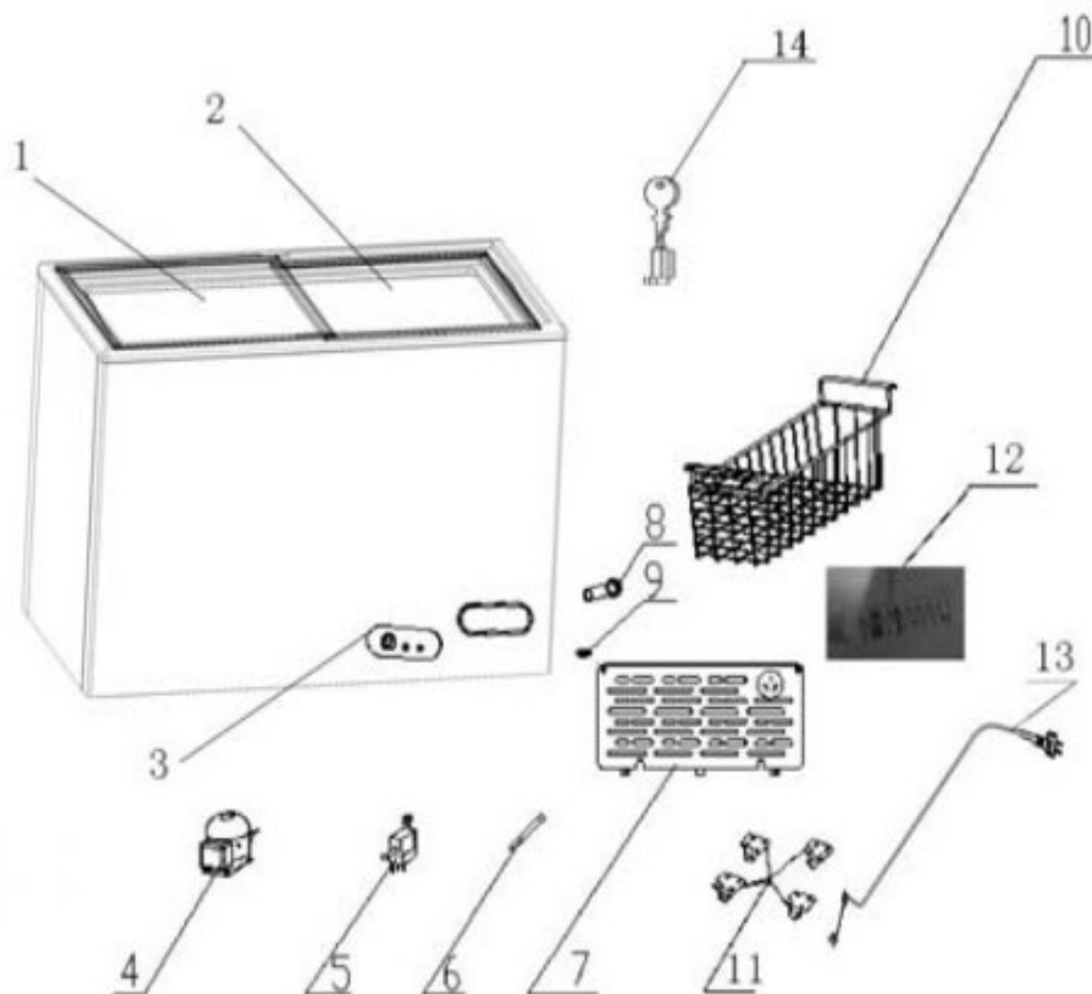
Explosion View Of KCNF073WS
