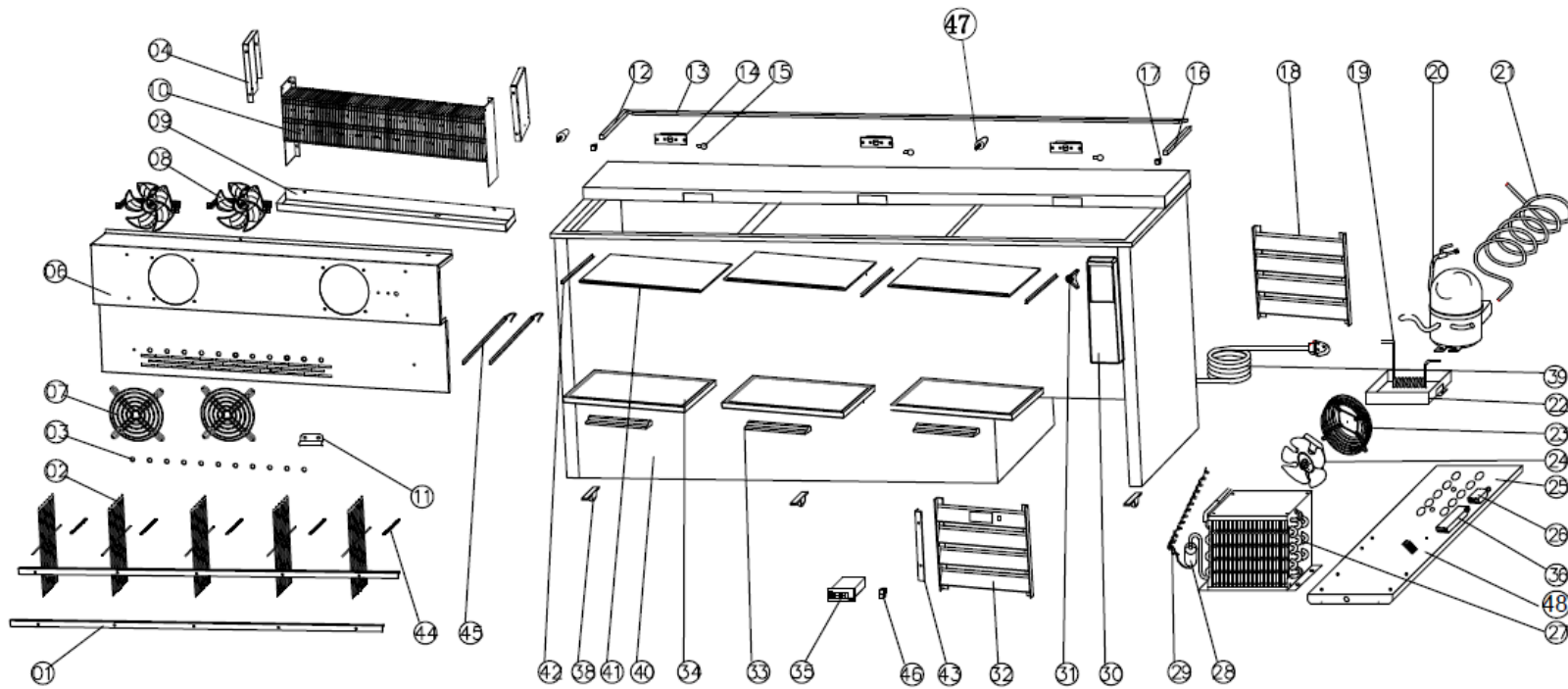
EXPLODE DRAWING OF KCHBC95
