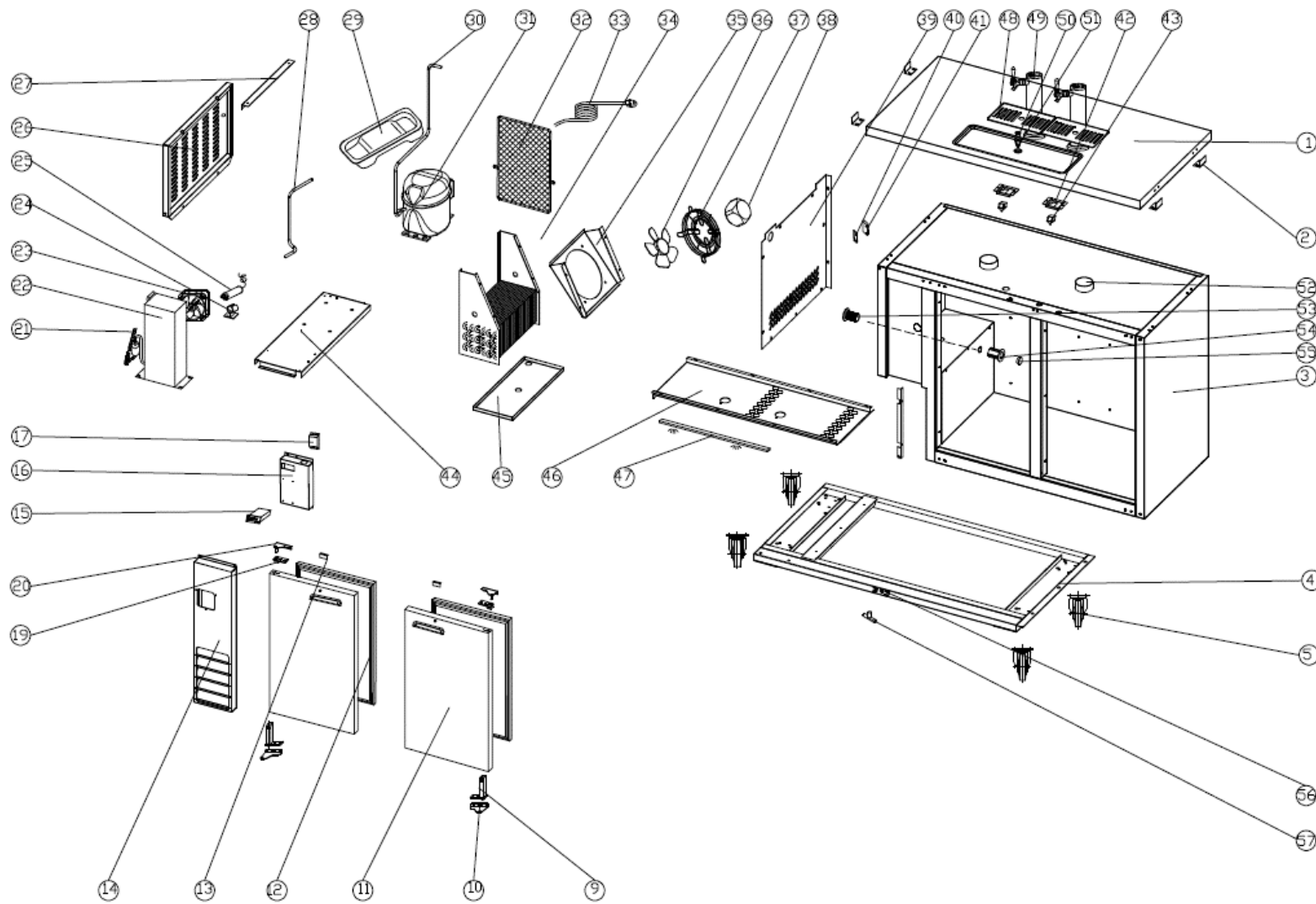
EXPLODE DRAWING OF KCHBBD2D2T
