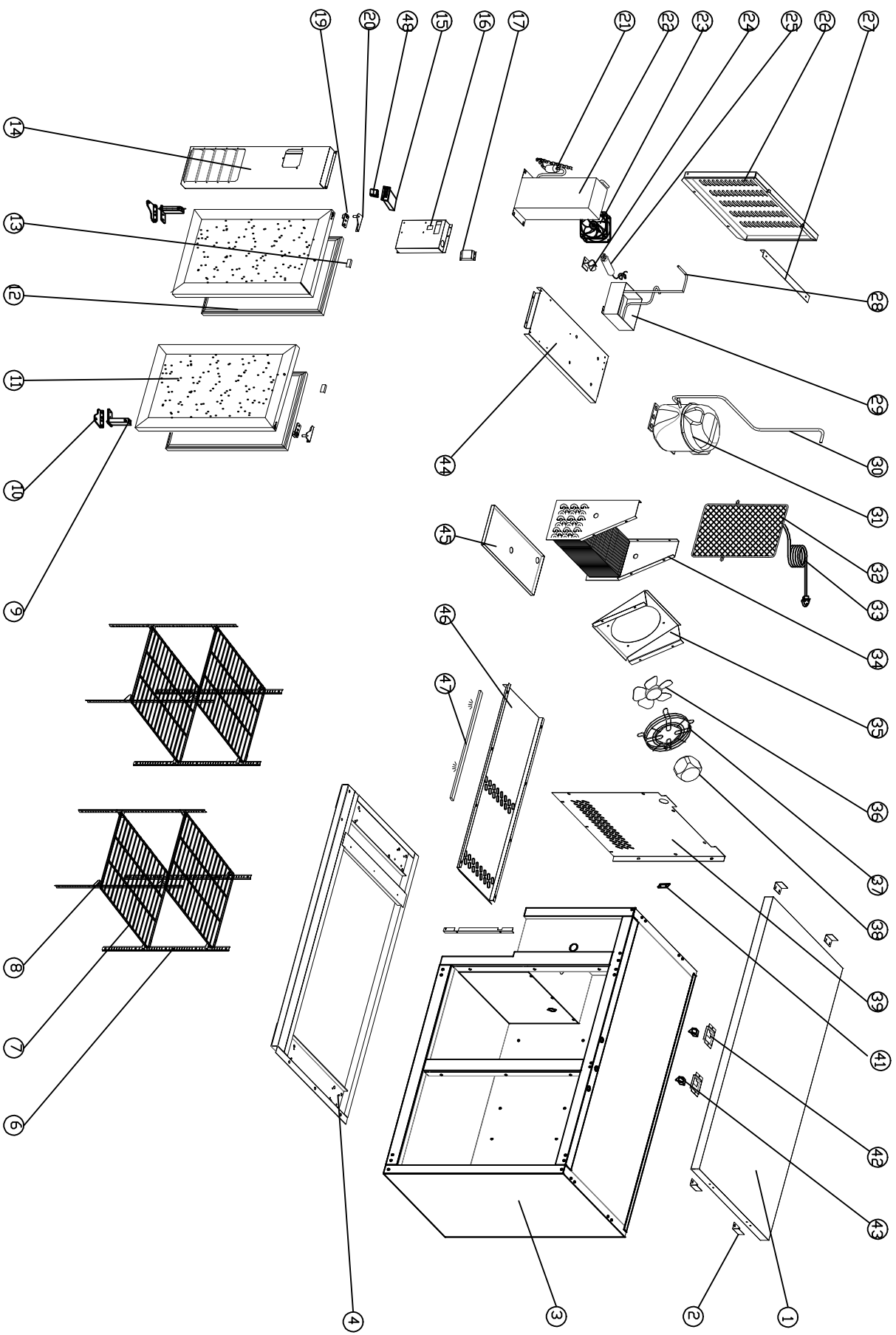
EXPLODE DRAWING OF KCHBB48G
