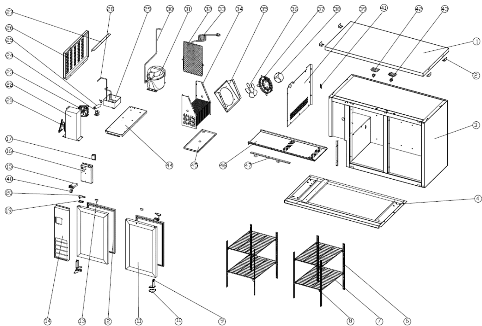
EXPLODE DRAWING OF KCHBB48G
